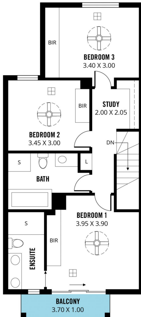
UPPER FLOOR
