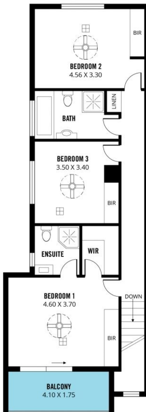
UPPER FLOOR
