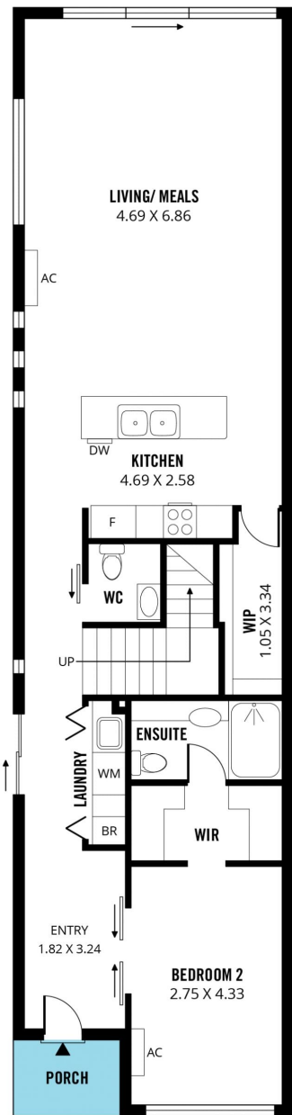
GROUND FLOOR
