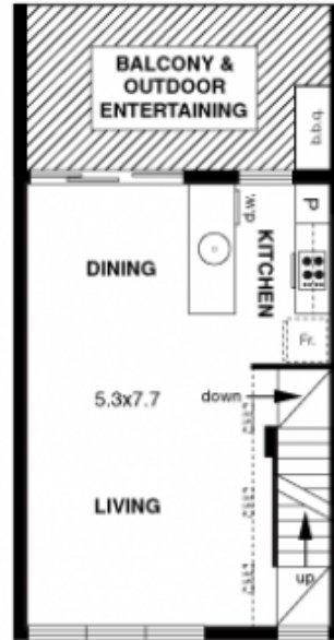
Second Level
