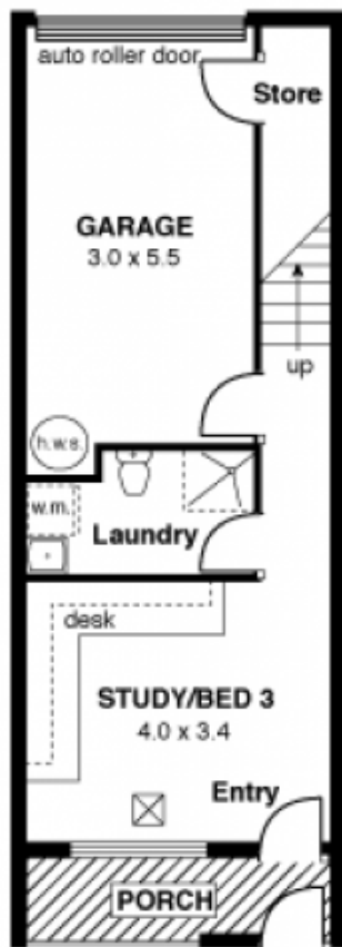
Ground Level
