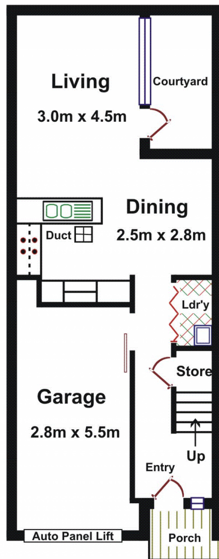
Lower Floor
