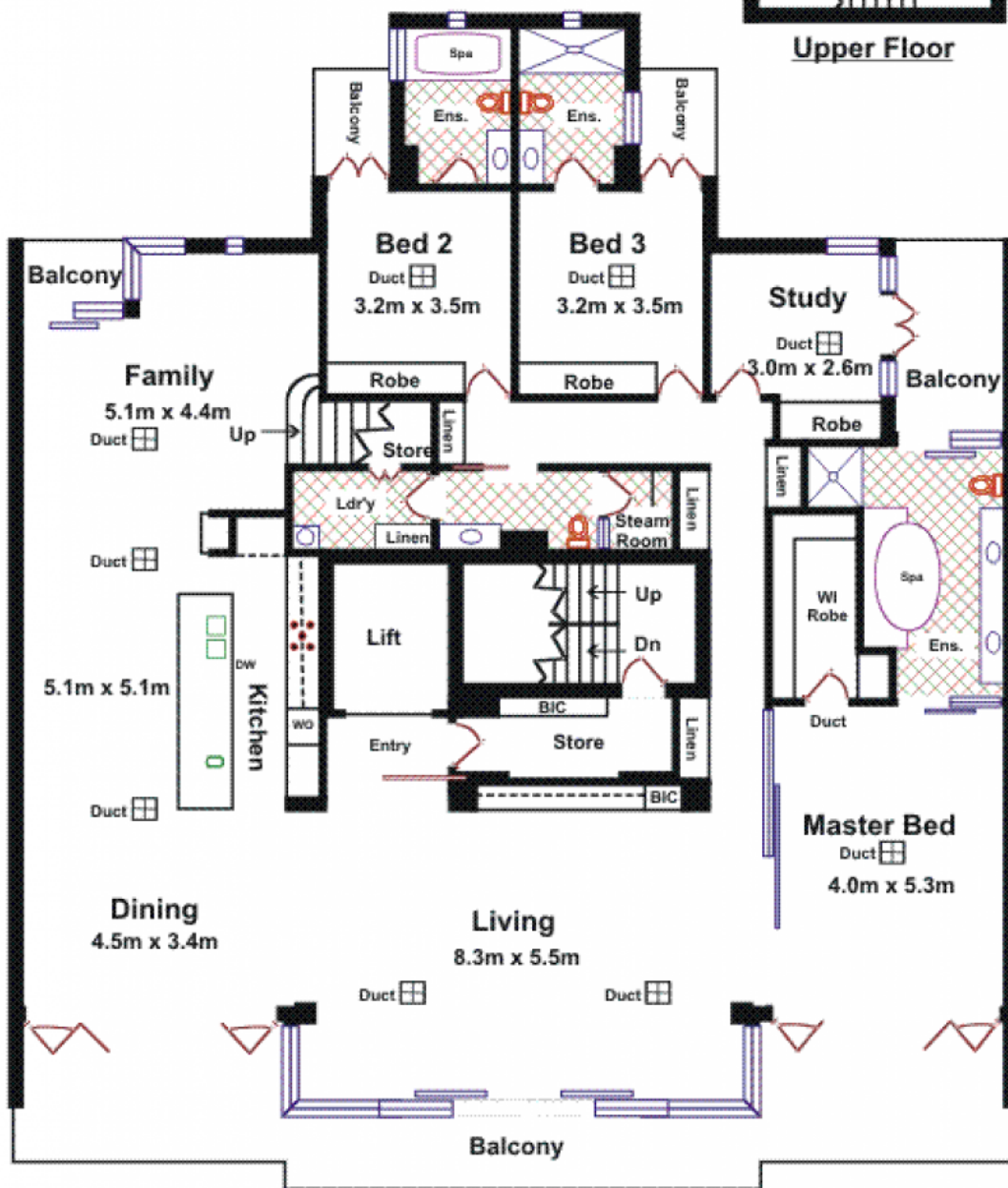
Lower Floor
