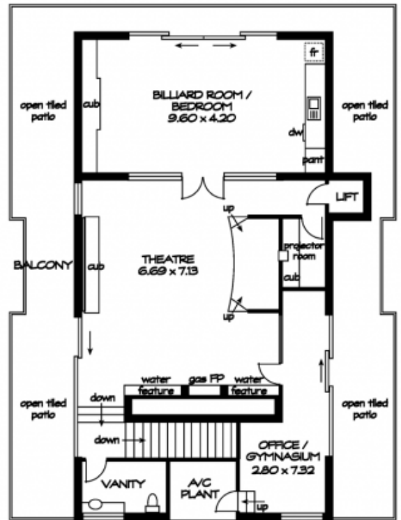
UPPER FLOOR (FOURTH FLOOR)
