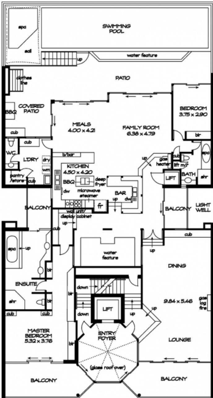
LOWER FLOOR (THIRD FLOOR)
