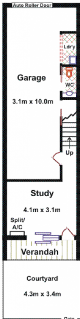
Ground Floor
