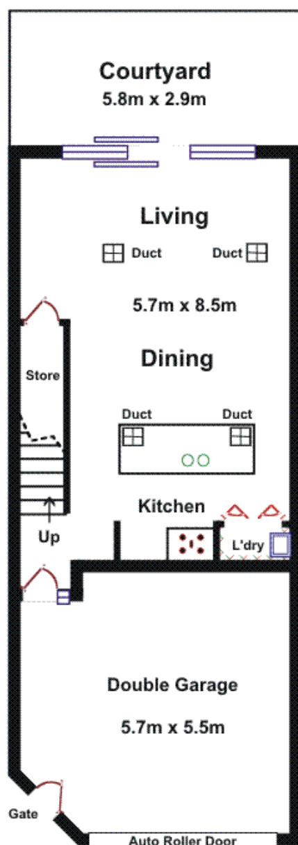
Lower Floor
