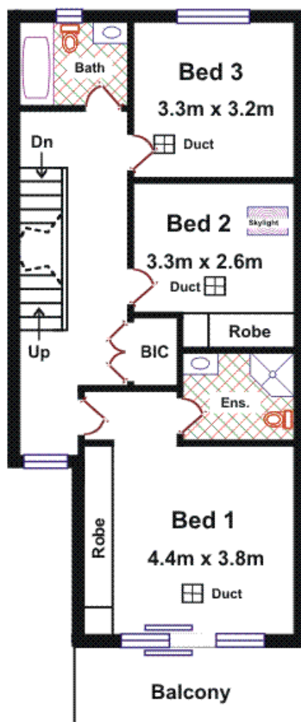
Upper Floor
