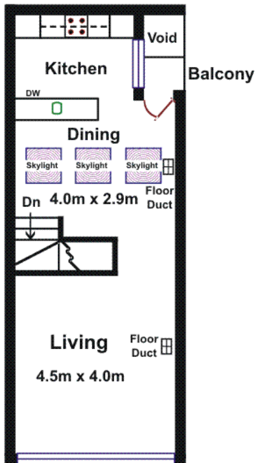
Upper Floor
