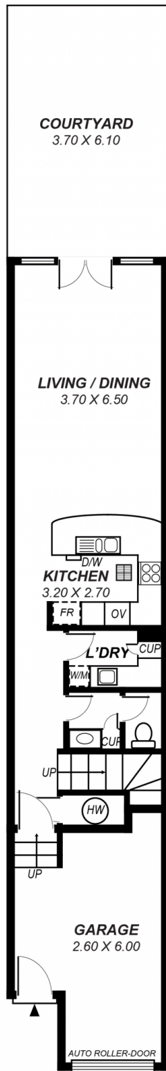
LOWER LEVEL
