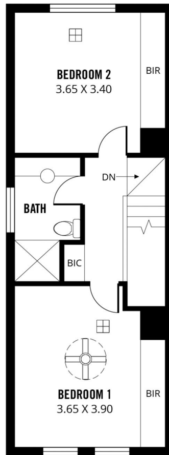
UPPER FLOOR
