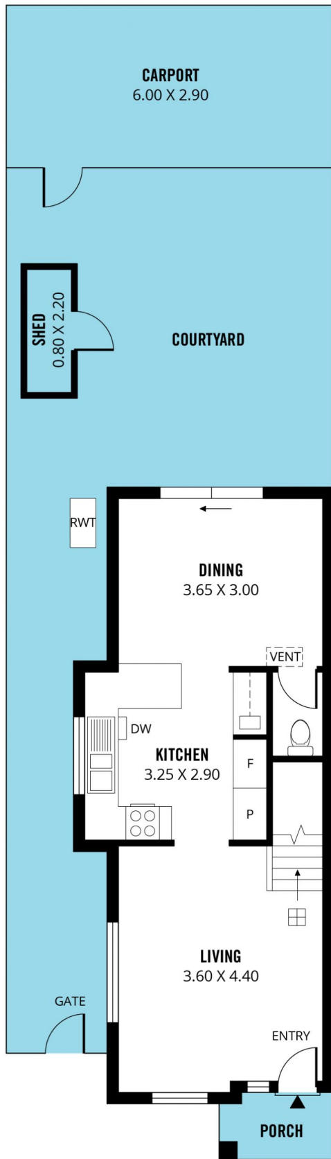
LOWER FLOOR
