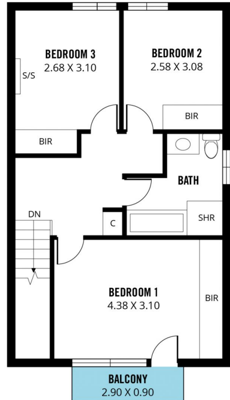
UPPER LEVEL
