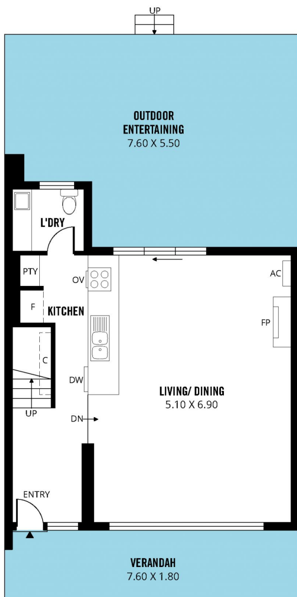
LOWER LEVEL
