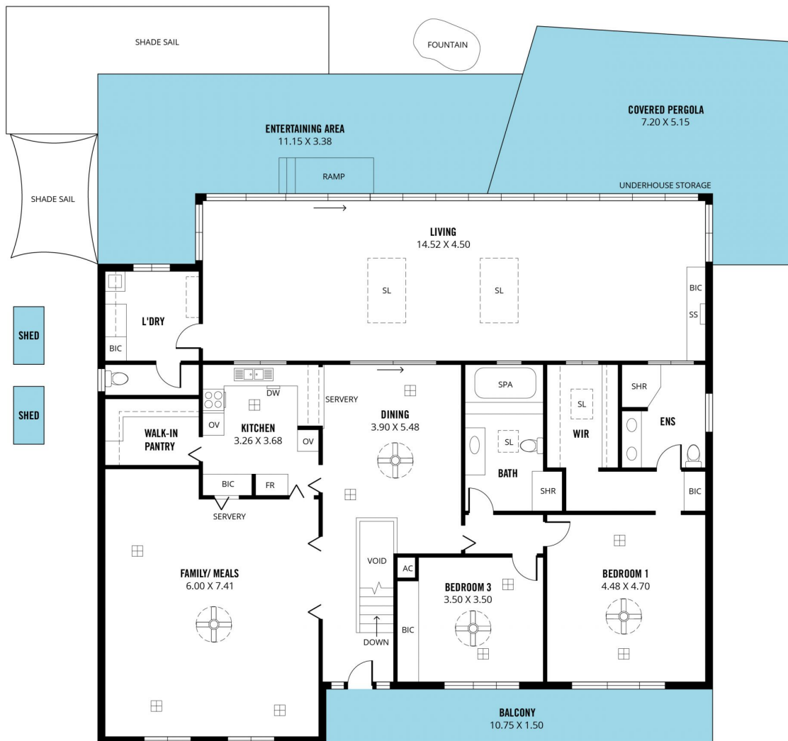
UPPER FLOOR
