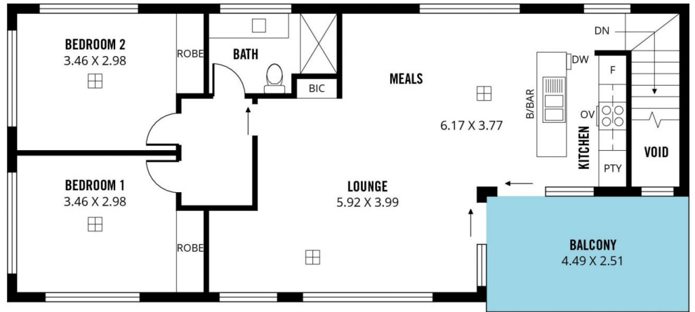
UPPER LEVEL
