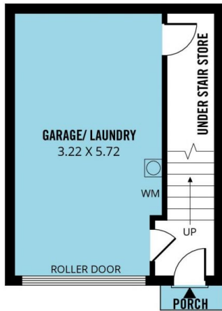
GROUND LEVEL
