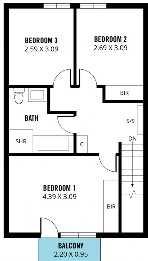
UPPER FLOOR
