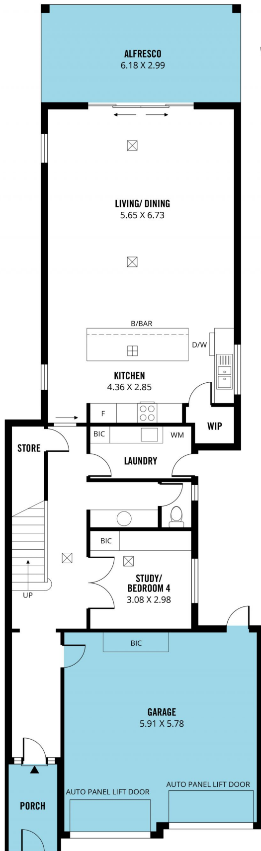
LOWER LEVEL
