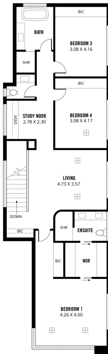
FIRST FLOOR
