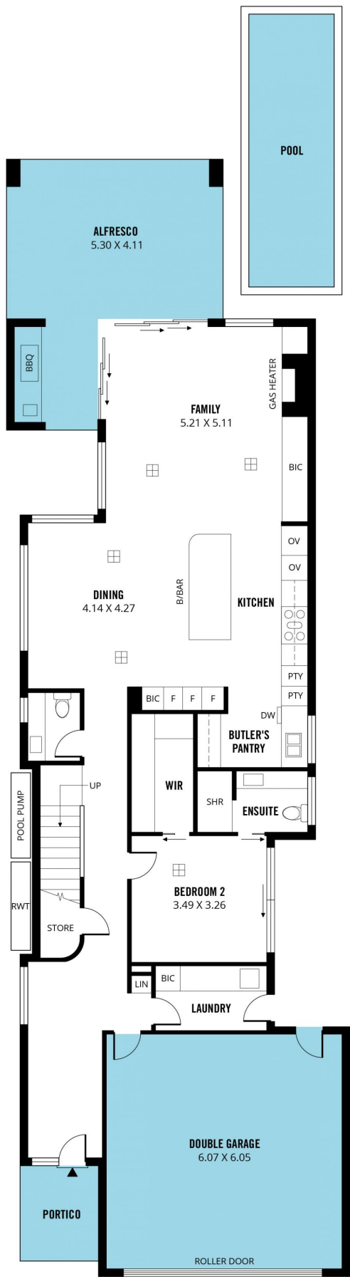
GROUND FLOOR
