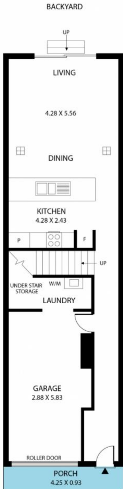
GROUND FLOOR
