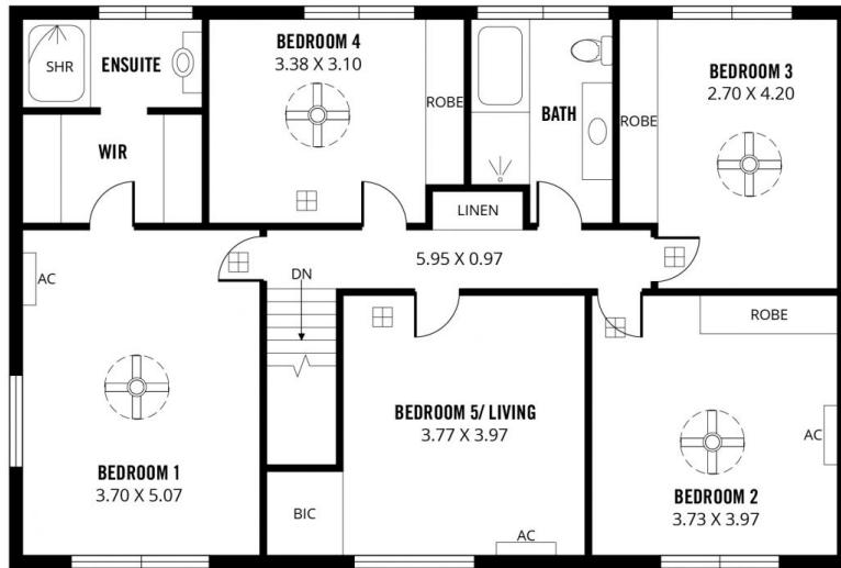
UPPER FLOOR
