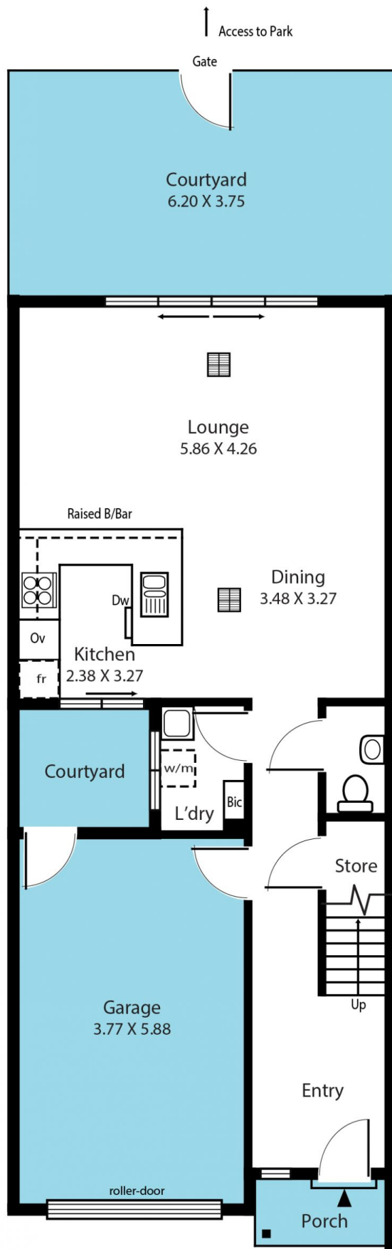
Ground Floor
