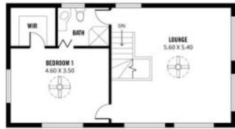
UPPER FLOOR
