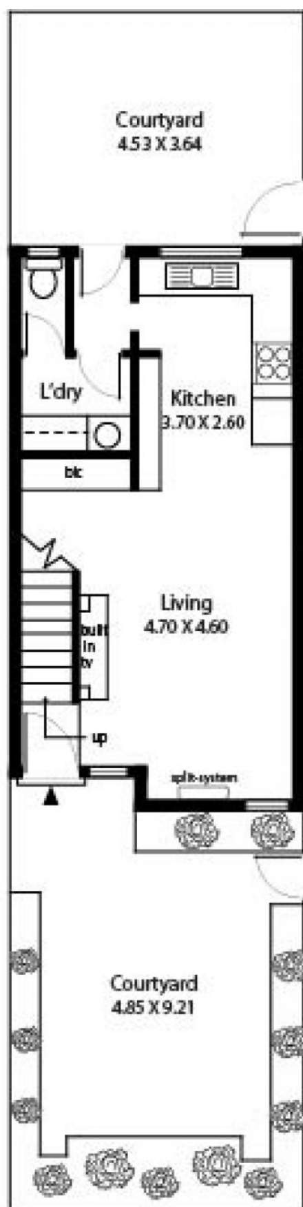
Ground floor
