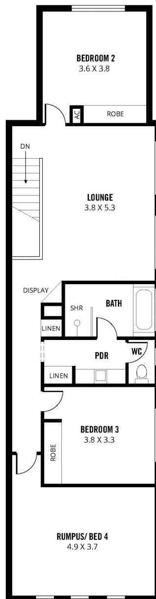
UPPER FLOOR
