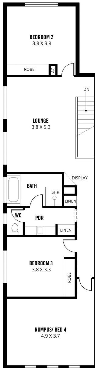
UPPER FLOOR
