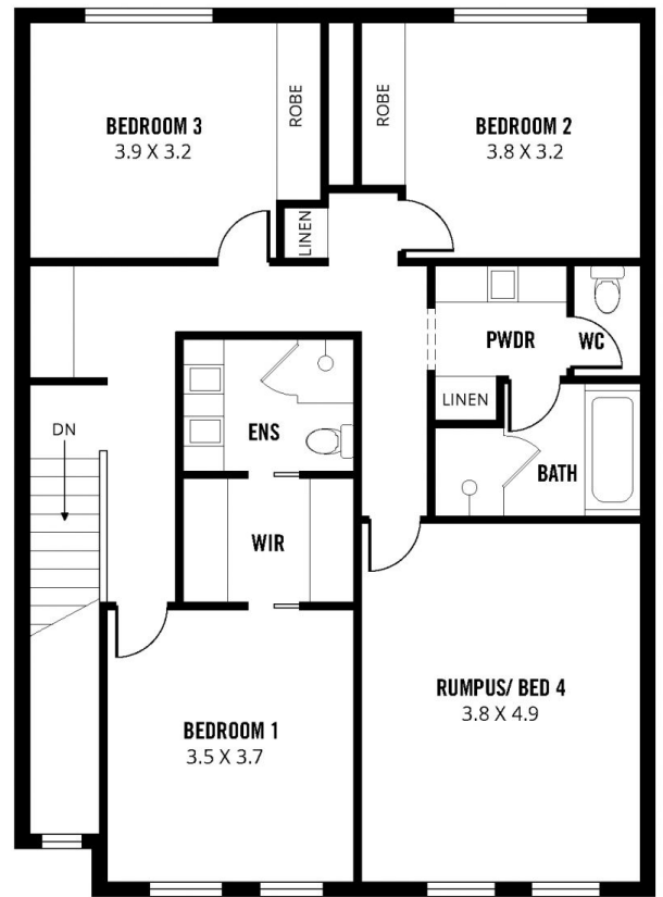
UPPER FLOOR
