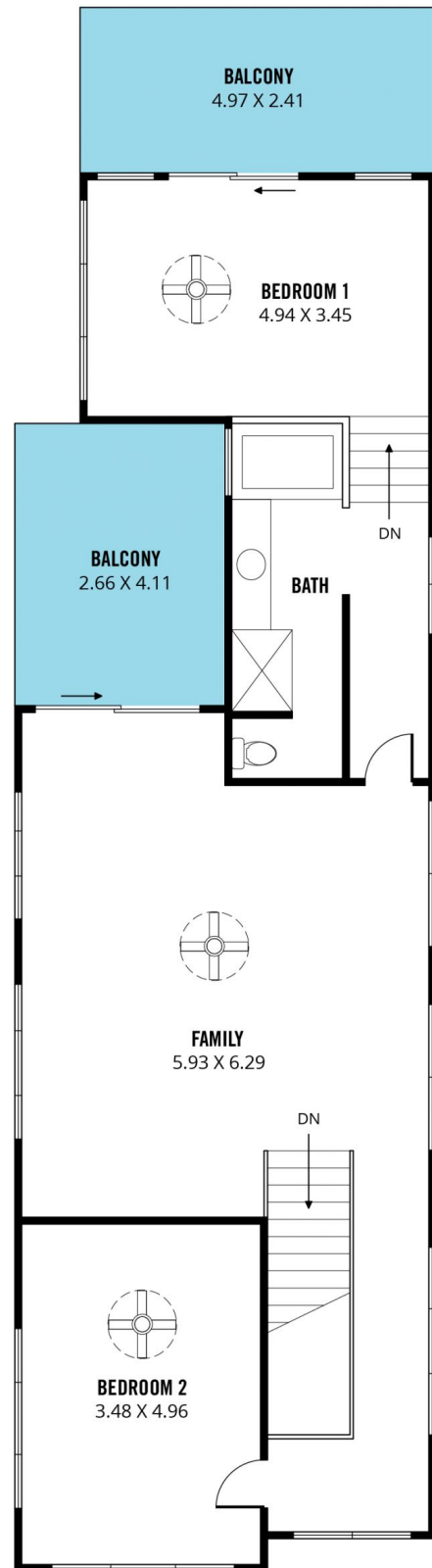
UPPER FLOOR PLAN
