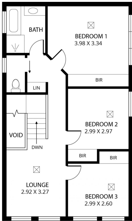
UPPER LEVEL
