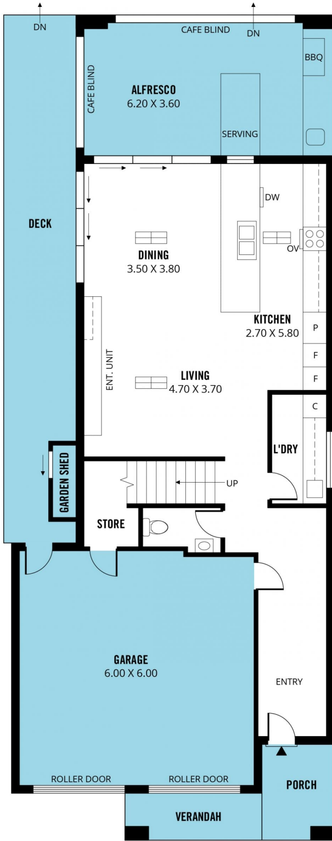
GROUND LEVEL
