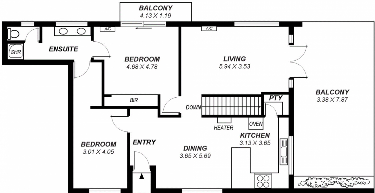
UPPER FLOOR
