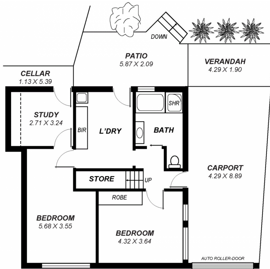
LOWER FLOOR
