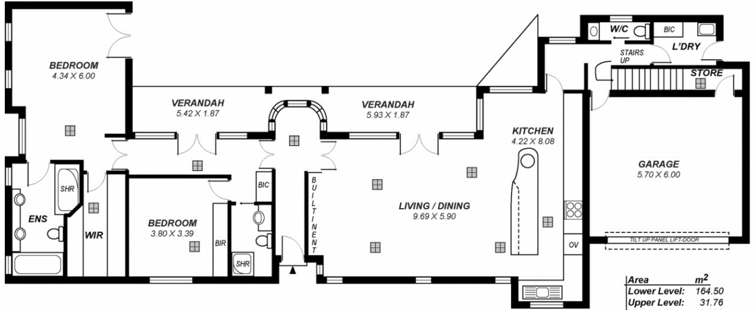
LOWER LEVEL
