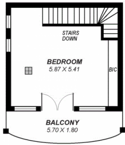
UPPER LEVEL
