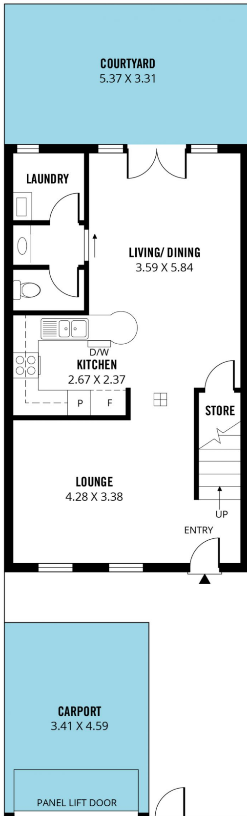
GROUND FLOOR
