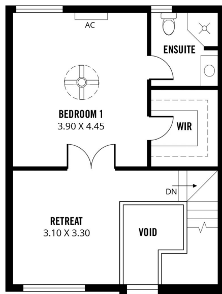
UPPER FLOOR
