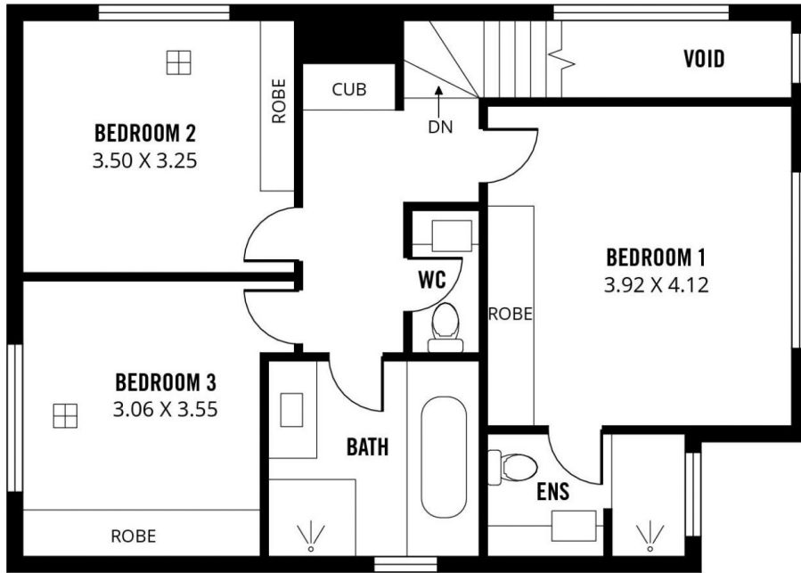
UPPER FLOOR
