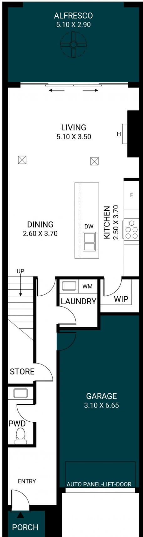
GROUND FLOOR
