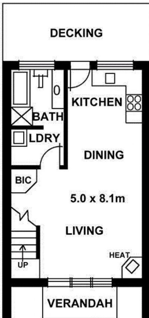
GROUND FLOOR
