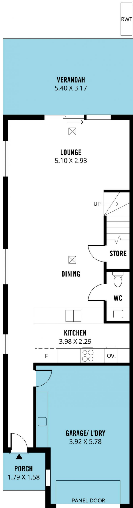
GROUND FLOOR
