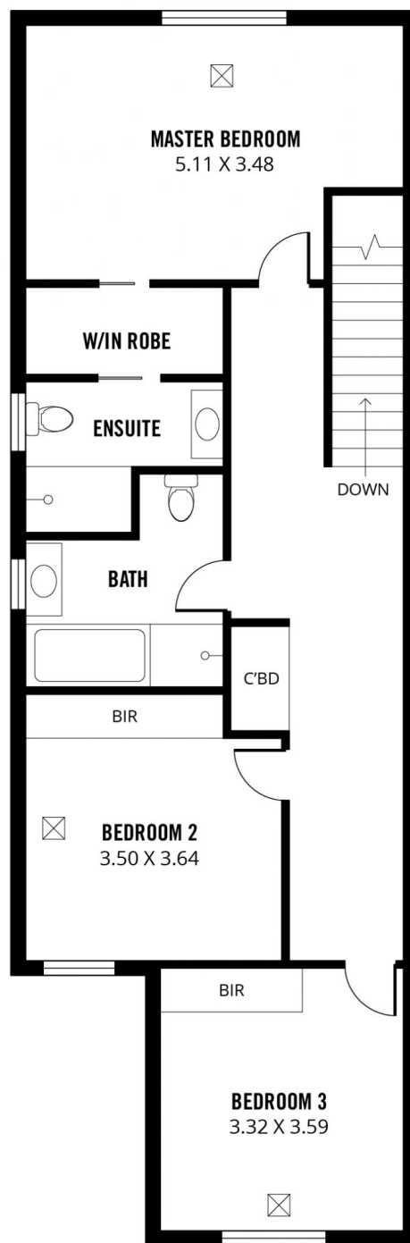
SECOND FLOOR
