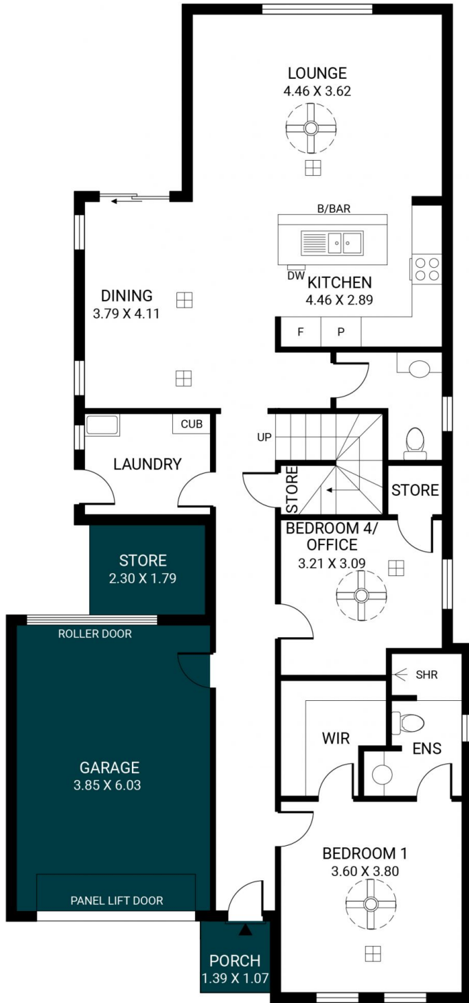
LOWER LEVEL
