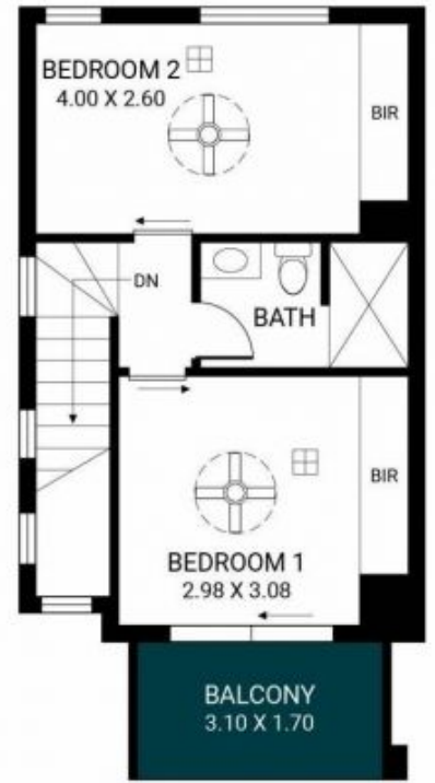
SECOND LEVEL
